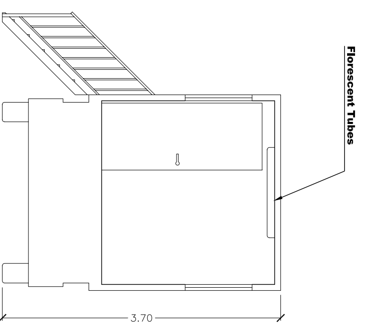
SECTION-02
